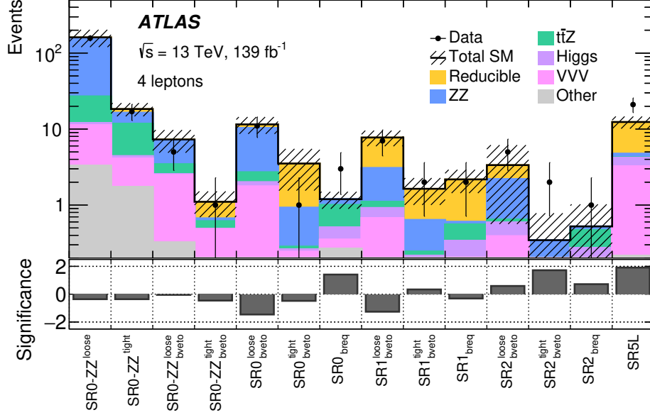
Figure 7: Expected and observed yields in the signal regions after the background-only fit. “Other” is the sum of the t\bar{t}WZ , t\bar{t}WW , t\bar{t}ZZ , t\bar{t}WH , t\bar{t}HH , t\bar{t}tW , and t\bar{t}t\bar{t} backgrounds. Both the statistical and systematic uncertainties in the SM background are included in the uncertainties shown. The significance of any difference between observed and expected yields is shown in the bottom panel, calculated with the profile likelihood method from Ref. [119].
