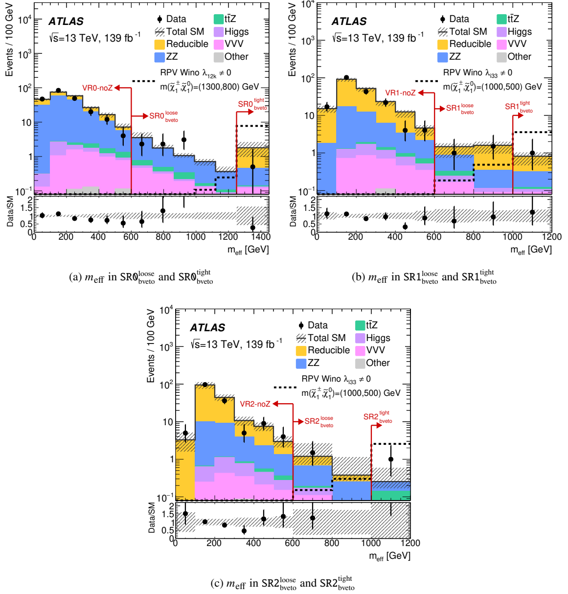
Figure 9: The m_{\text{eff}} distribution in (a) \text{SR0}_{\text{bveto}}^{\text{loose}} and \text{SR0}_{\text{bveto}}^{\text{tight}} , (b) \text{SR1}_{\text{bveto}}^{\text{loose}} and \text{SR1}_{\text{bveto}}^{\text{tight}} , and (c) \text{SR2}_{\text{bveto}}^{\text{loose}} and \text{SR2}_{\text{bveto}}^{\text{tight}} for events passing the signal region requirements except the m_{\text{eff}} requirement. Distributions for data, the estimated SM backgrounds after the background-only fit, and an example SUSY scenario are shown. “Other” is the sum of the t\bar{t}WZ , t\bar{t}WW , t\bar{t}ZZ , t\bar{t}WH , t\bar{t}HH , t\bar{t}tW , and t\bar{t}t\bar{t} backgrounds. The last bin captures the overflow events. The lower panel shows the ratio of the observed data to the expected SM background yield in each bin. Both the statistical and systematic uncertainties in the SM background are included in the shaded band. The red arrows indicate the m_{\text{eff}} selections in the signal and validation regions.
