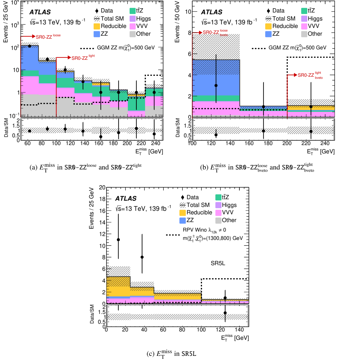
Figure 8: The E_T^{\text{miss}} distribution in (a) SR0-ZZ loose and SR0-ZZ tight , (b) SR0-ZZ loose bveto and SR0-ZZ tight bveto , and (c) SR5L for events passing the signal region requirements except the E_T^{\text{miss}} requirement. Distributions for data, the estimated SM backgrounds after the background-only fit, and an example SUSY scenario are shown. “Other” is the sum of the tWZ , t\bar{t}WW , t\bar{t}ZZ , t\bar{t}WH , t\bar{t}HH , t\bar{t}tW , and t\bar{t}t\bar{t} backgrounds. The last bin captures the overflow events. The lower panel shows the ratio of the observed data to the expected SM background yield in each bin. Both the statistical and systematic uncertainties in the SM background are included in the shaded band. The red arrows indicate the E_T^{\text{miss}} selections in the signal regions.
