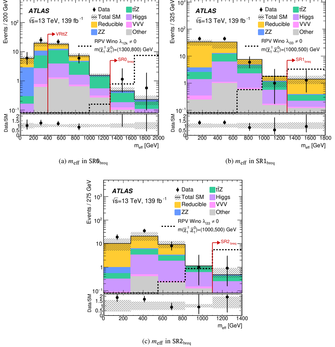
Figure 10: The m_{\text{eff}} distribution in (a) \text{SR0}_{\text{breq}} , (b) \text{SR1}_{\text{breq}} , and (c) \text{SR2}_{\text{breq}} for events passing the signal region requirements except the m_{\text{eff}} requirement. Distributions for data, the estimated SM backgrounds after the background-only fit, and an example SUSY scenario are shown. “Other” is the sum of the tWZ , t\bar{t}WW , t\bar{t}ZZ , t\bar{t}WH , t\bar{t}HH , t\bar{t}tW , and t\bar{t}t\bar{t} backgrounds. The last bin captures the overflow events. The lower panel shows the ratio of the observed data to the expected SM background yield in each bin. Both the statistical and systematic uncertainties in the SM background are included in the shaded band. The red arrows indicate the m_{\text{eff}} selections in the signal and validation regions.
